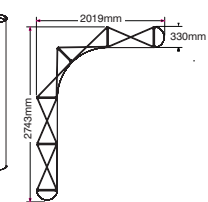
3m large "L Shaped Pop-Up" exhibit kit
