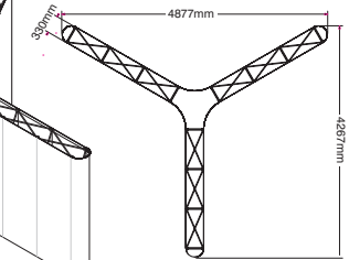
6m star exhibit kit
