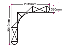
3m small "L Shaped Pop-Up" exhibit kit
