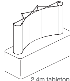
2.4m tabletop kit footprint dimensions: 1495mm h x 2540mm w x 685mm d
